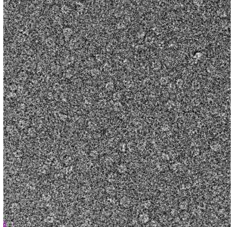
SR398+ \alpha\beta +GroES+ATP
